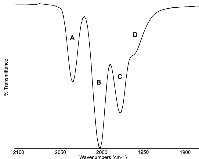
Figure 2. Representative metal carbonyl IR spectra for complexes 10a–16b .
